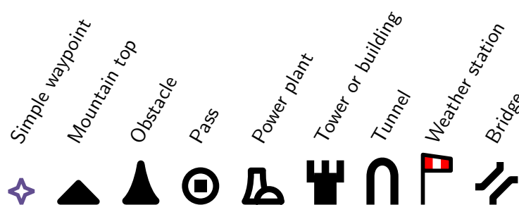
Figure 4.1: non-landables
