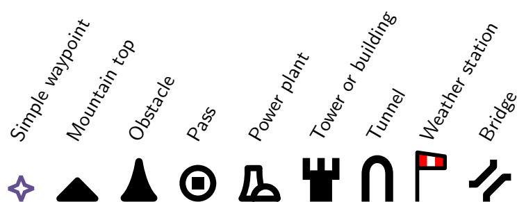
Figure 4.1: non-landables
